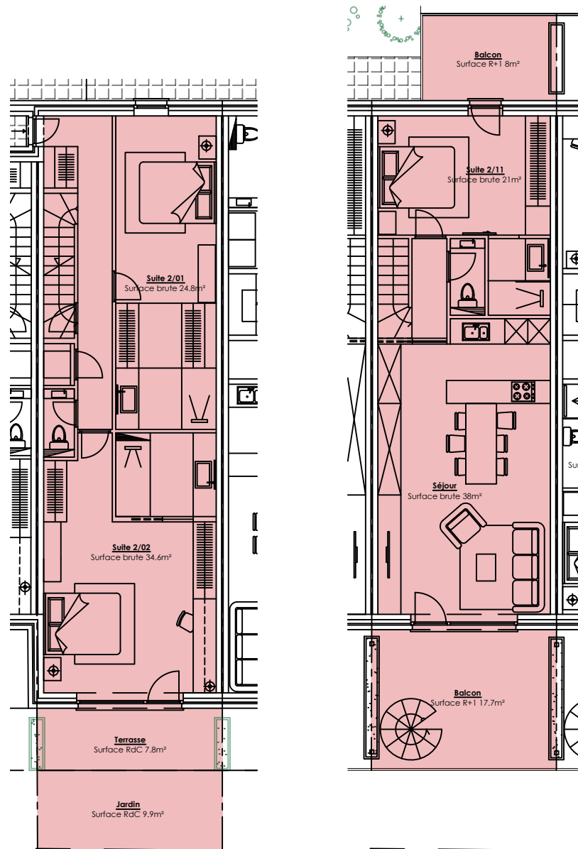
Maison 2 - PMR Surface brute RdC: 77.2m 2 Surface brute totale: 143.7m 2 Surface totale extérieure: 43.4m 2
