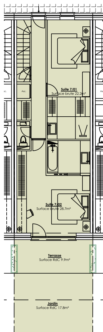
Maison 7 Surface brute RdC 66.5m 2 Surface brute totale 210.5m 2 Surface totale extérieure 63.7m 2
