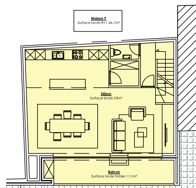
Plan R+1
